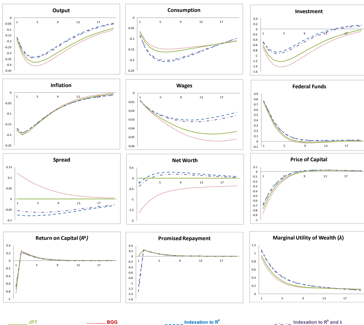
Figure 3.d. Impulse Response Functions to a One Standard Deviation Monetary Policy Shock Keeping parameters constant to the R^k indexation model except R^k and lambda indexation parameters ( \phi_k and \lambda )
