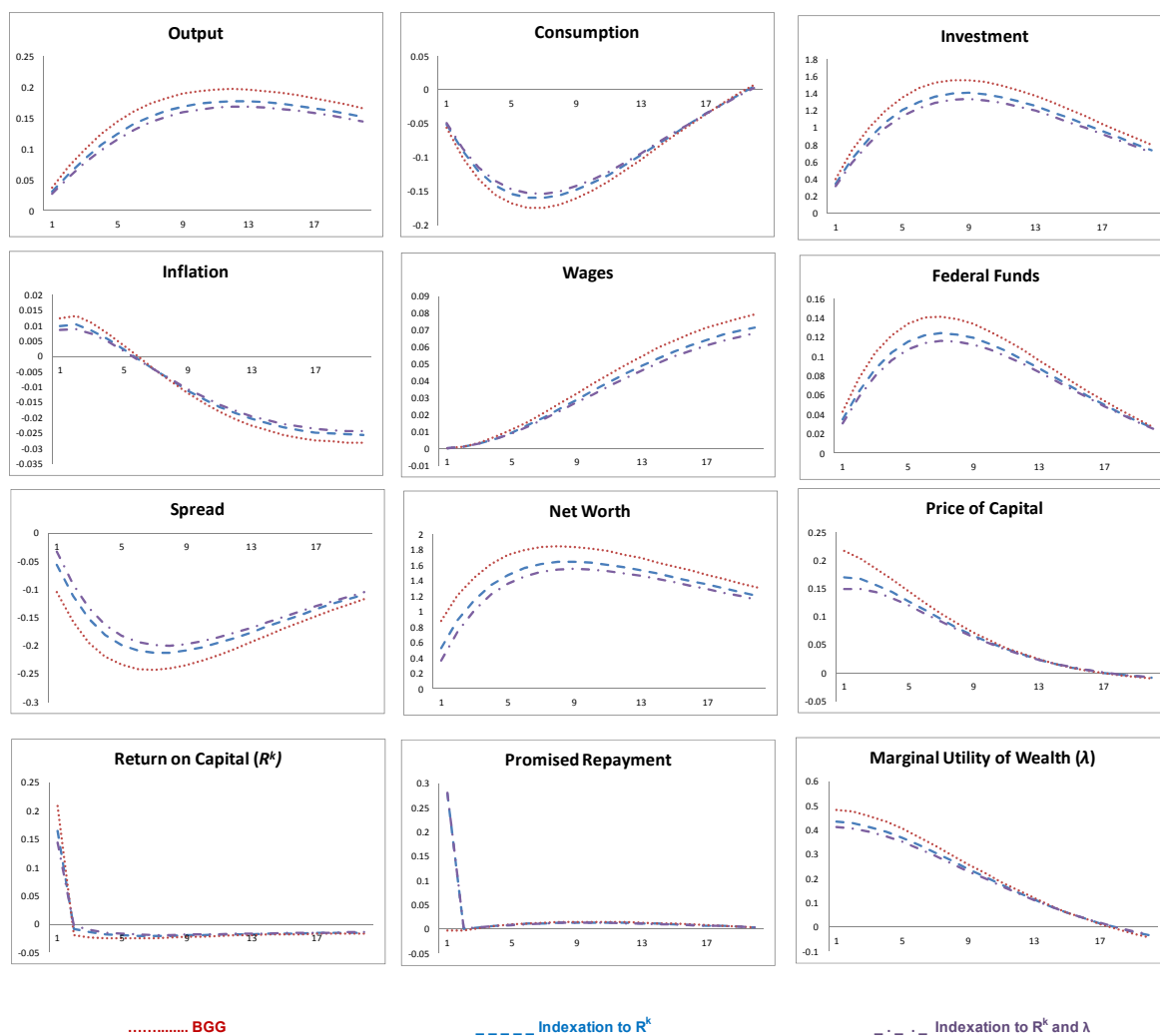
Figure 3.b. Impulse Response Functions to a One Standard Deviation Net Worth Shock Keeping parameters constant to the R^k indexation model except R^k and lambda indexation parameters ( \chi_R and \chi_\lambda )
