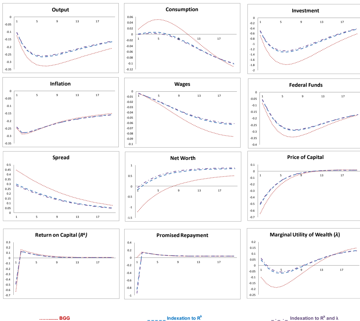
Figure 3.c. Impulse Response Functions to a One Standard Deviation Idiosyncratic Variance Shock Keeping parameters constant to the R^* indexation model except R^* and lambda indexation parameters ( \lambda_R and \lambda_\lambda )
