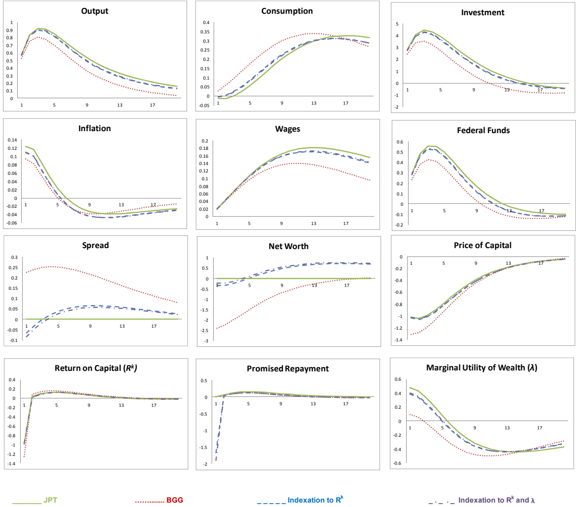
Figure 3.a. Impulse Response Functions to a One Standard Deviation Marginal Efficiency of Investment Shock Keeping parameters constant to the R^k indexation model except R^k and lambda indexation parameters ( \lambda_k and \lambda )
